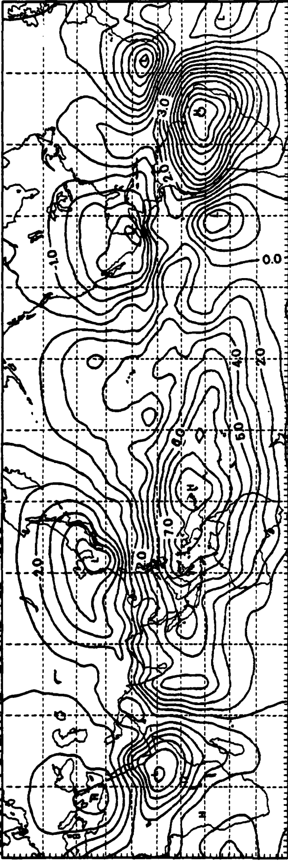
VELOCITY POTENTIAL 200MB FEB 1980
